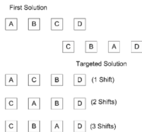
Figure 1. Path Relinking (Goldberg Et Al, 2008)
