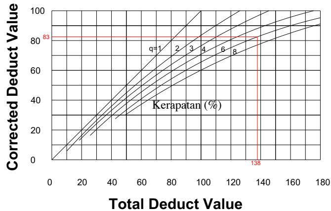
Gambar 5. Grafik penentuan CDV (ASTM internasional, 2007)
